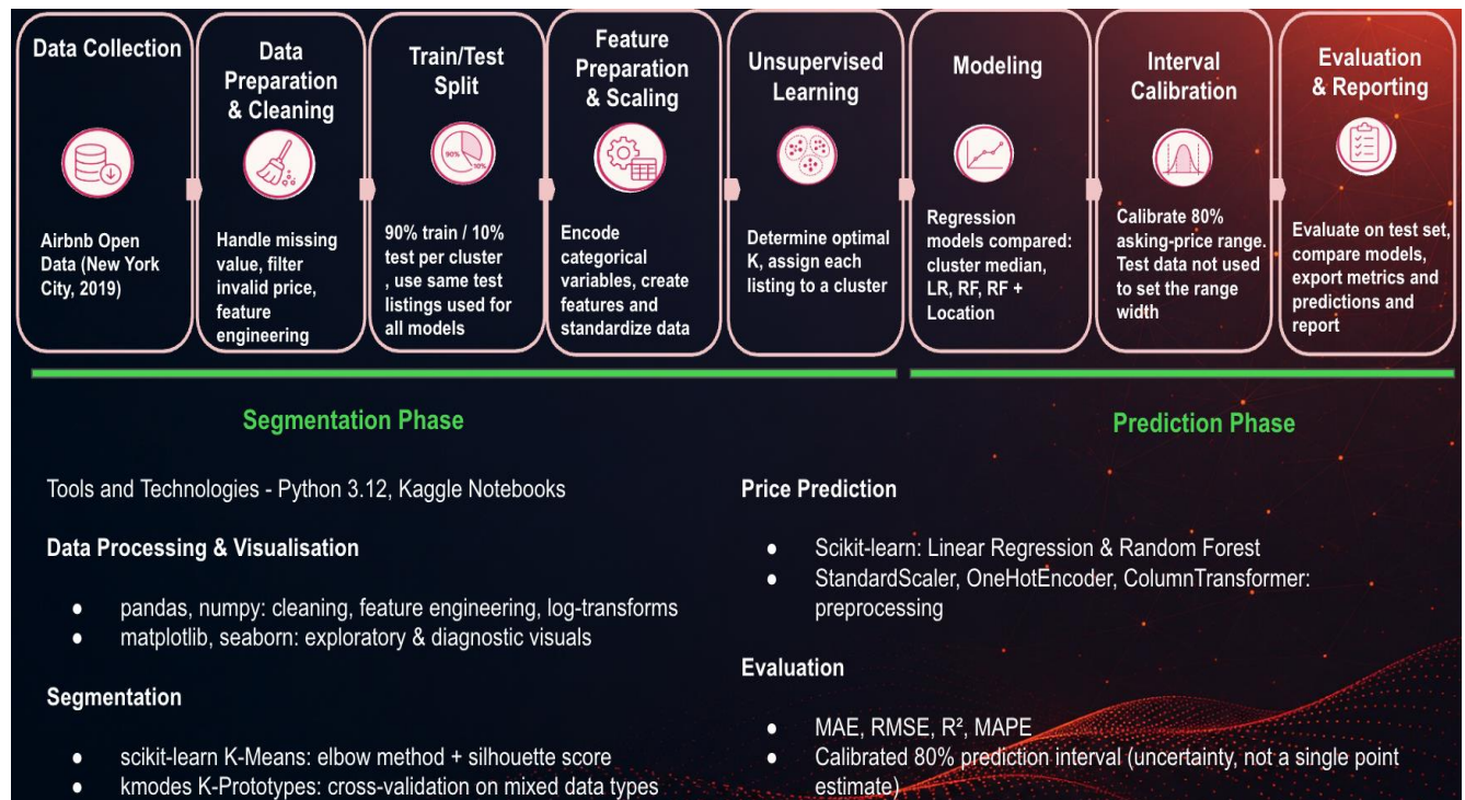
Figure 2. Analytical Pipeline and tooling used for Airbnb Segmentation and Price Prediction. Source: Authors' own work.
