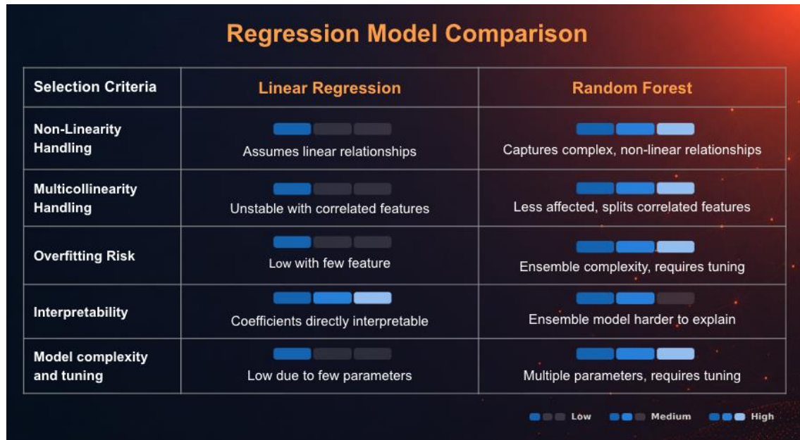
Figure 9. Comparison of Regression Models. Source: Developed by the authors, based on Hastie, Tibshirani and Friedman (2009)
